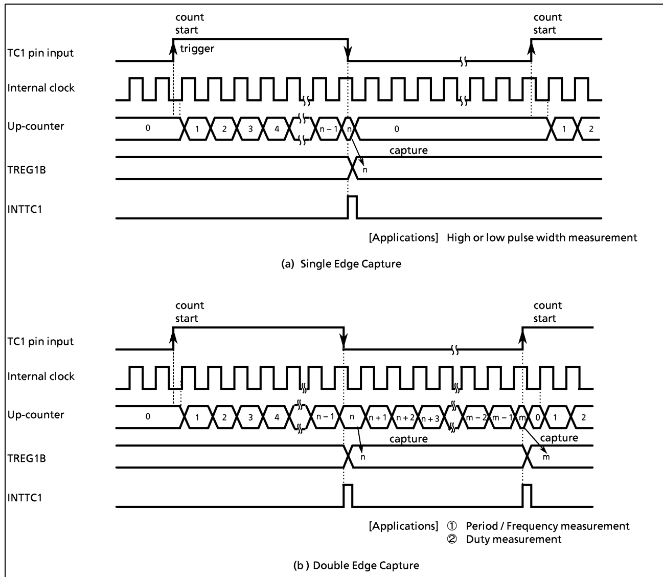
Figure 2-17. Pulse Width Measurement Mode Timing Chart
