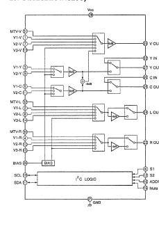
4-4. IC BLOCK DIAGRAMS A BOARD IC1261 MM1311AD (KV-27S20/29RS20C/29SD1/29RS20/29PS1/32S20/34RS20C)
