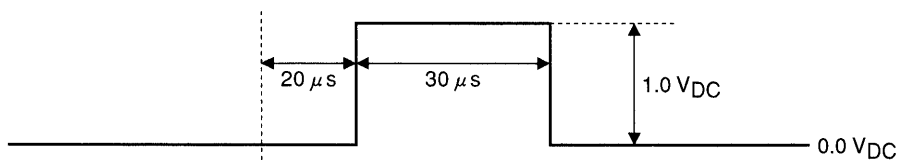
RGB input signal 2 (O-2)
