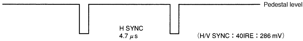
XIRE signal (L-X)
