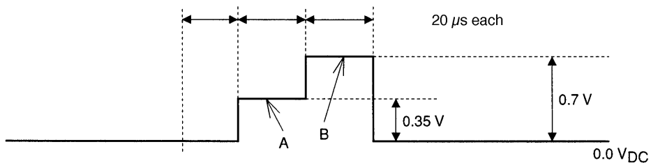
RGB input signal 2 (O-2)
