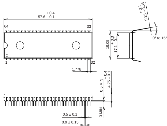
64PIN SDIP (PLASTIC) 750mil
